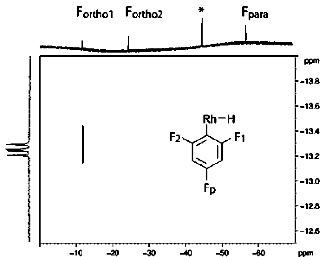
Figure 4. ^1\text{H}-^{19}\text{F} HETCOR NMR spectra (400 MHz) of 4 showing that one ortho fluorine is coupled to the hydride. ^1\text{H} (hydride region) and ^{19}\text{F} NMR spectra for 4 are plotted along the y- and x-axes, respectively. * indicates free \text{C}_6\text{H}_3\text{F}_3 .
