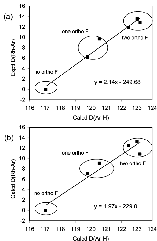
Figure 8. Plot of relative Rh–C aryl bond strength vs calculated C–H bond strength (kcal mol −1 ). (a) Experimentally determined D(\text{Rh}-\text{C}_{\text{aryl}}) and (b) DFT-calculated D(\text{Rh}-\text{C}_{\text{aryl}}) .
