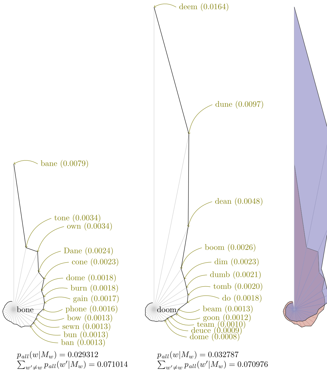
Fig. 4. The distribution of competitors for the words “bone” and “doom.” In the left and center panels, the 32 closest competitors for both words are shown in descending order of similarity, moving clockwise from the top; the length of the line for competitor w' is p(w'|w) . The 13 closest competitors for each word are labeled, along with their confusion probabilities (under the HMM-based p_{all} measure); for context, the p_{all} probability of getting the word right is also shown. In the right panel, the two distributions are superimposed, illustrating that substantially more of the competition for “doom” comes from the top 8 competitors, while “bone” has competition that is much more evenly distributed throughout the 32 competitors.
