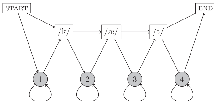
Fig. 2. The Hidden Markov Model for the word “cat.”
